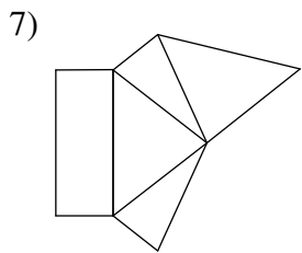
rectangular pyramid
