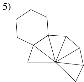
hexagonal pyramid
