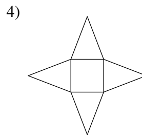
square pyramid
