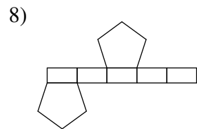
pentagonal prism
