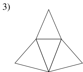
triangular pyramid
